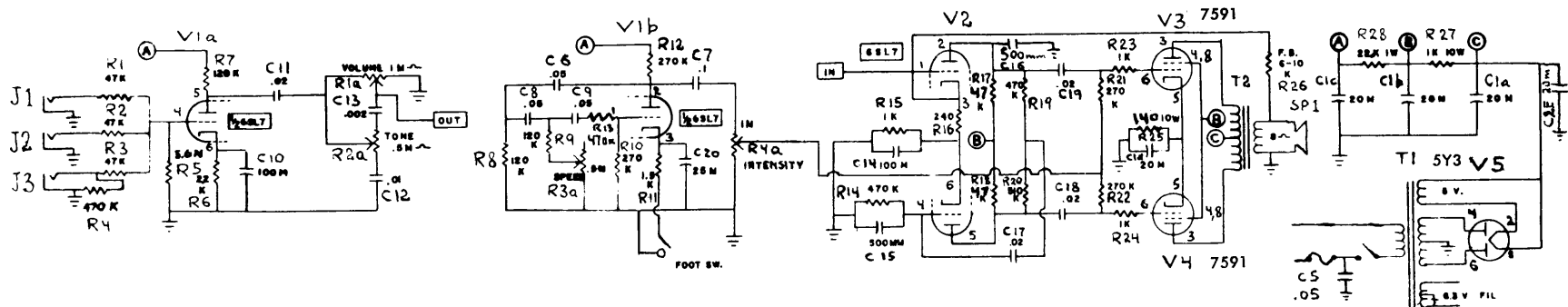
MODEL NO. R-12-A Tube Location (from left to right) 6SL7 6SL7 7591 7591 5Y3
