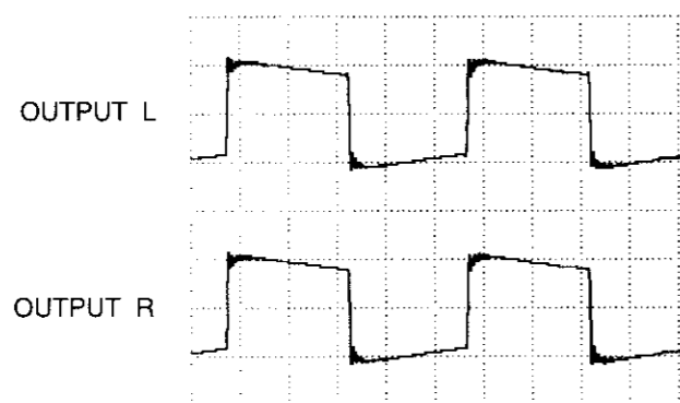
Fig.3/図3 (1mS/DIV, 0.1V/DIV)
