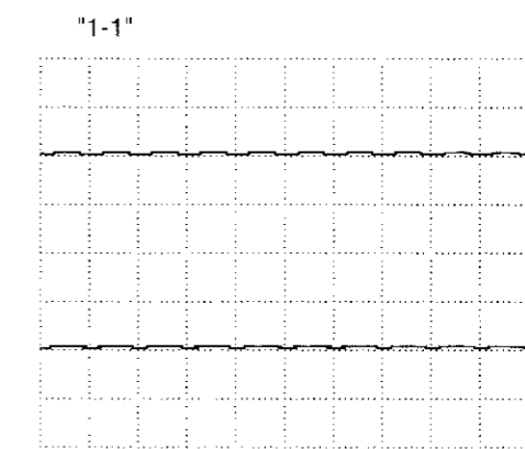
Fig.2/図2 (1mS/DIV, 0.1V/DIV)
