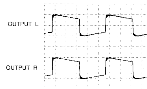
Fig4/図4 (1mS/DIV, 0.1V/DIV)
