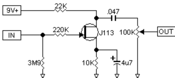
REDRAWN FROM ORIGINAL FACTORY SCHEMATIC
