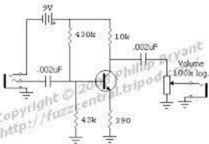
Electro Harmonix Screaming Bird/Screaming Tree drawn by Phillip Bryant http://fuzzcentral.tripod.com/
