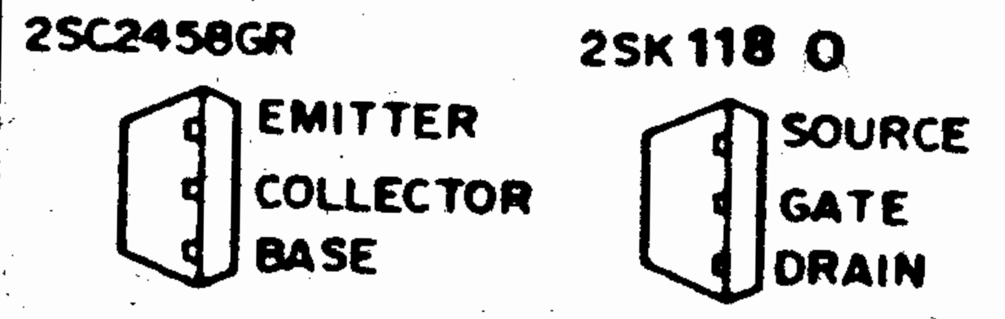
Bottom View
