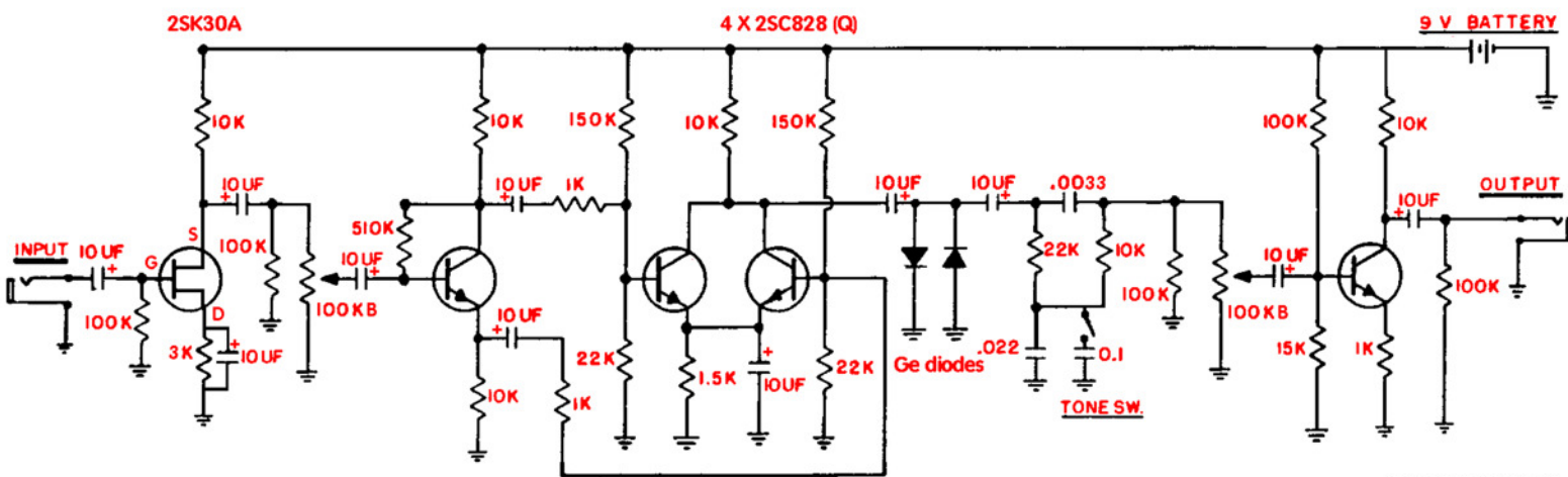
Fuzz section of an Ibanez STANDARD wah fuzz
