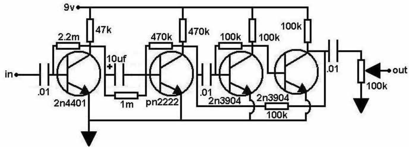
Confirmed schematic - Doug Deeper's RANDOM NUMBER GENERATOR, single knob version, posted with DD's permission, June 2006
