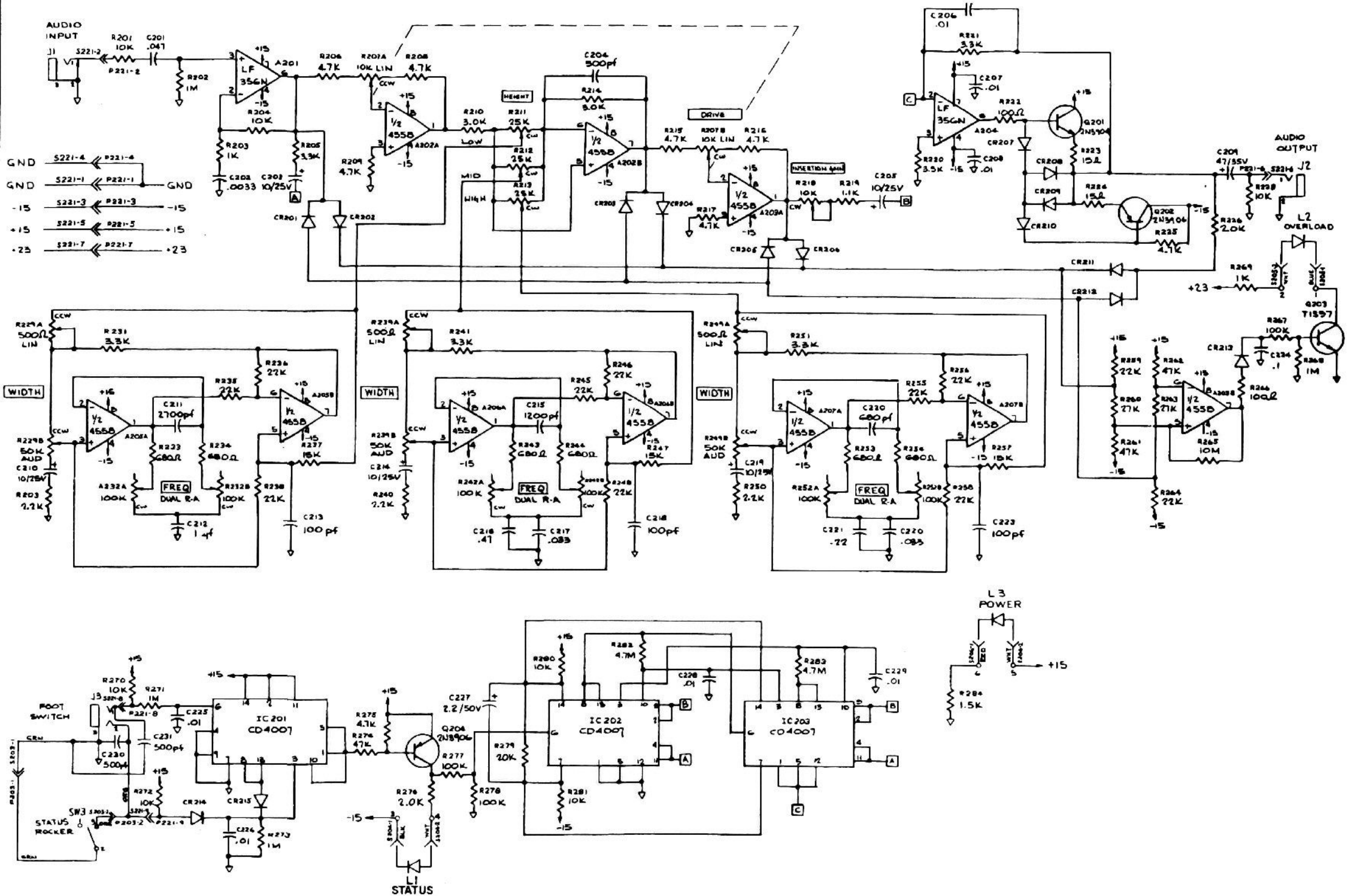
BOARD NO. 2 SIGNAL PROCESSOR PARAMETRIC EQUALIZER
