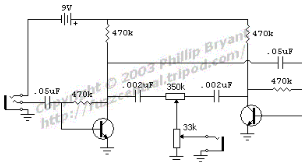
Mosrite Fuzz Rite drawn by Phillip Bryant http://fuzzcentral.tripod.com/
