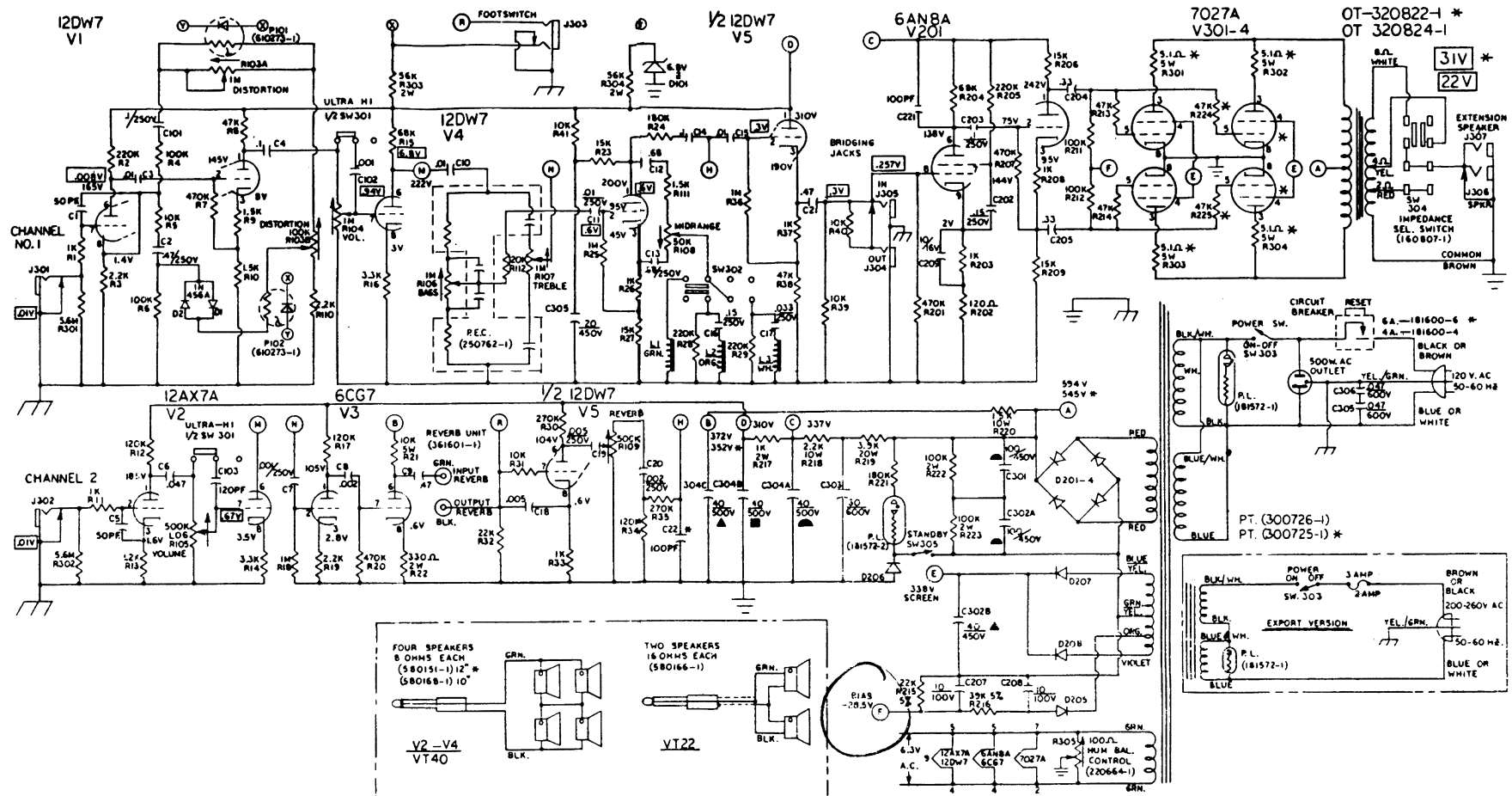
SCHMATIC (DISTORTION) V2/VT40/V4/VT22
