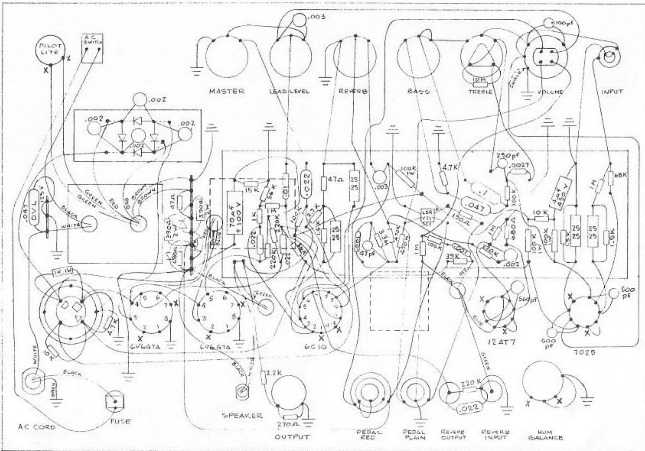
Fender Super Champ Amplifier Wiring Diagram
