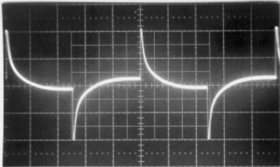
Fig. 9. Bass to 0.
