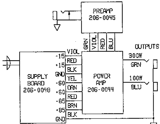
SUPPLY INTERCONNECTION DIAGRAM
