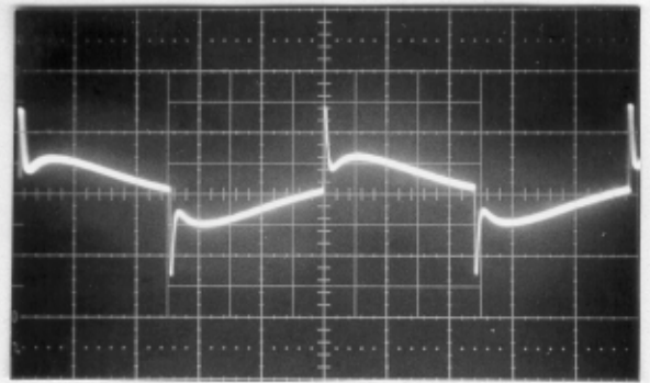
Fig. 5. Hi-Mid to 0.
