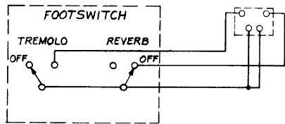
FOOTSWITCH & PLUG
