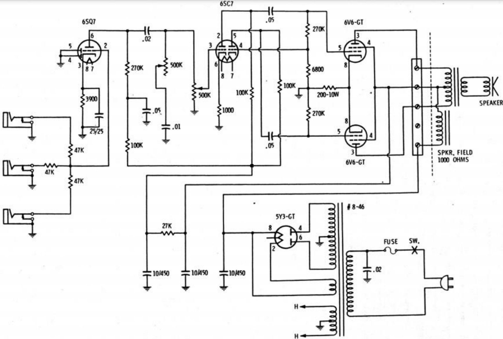
Gretsch Model G6155/6156
