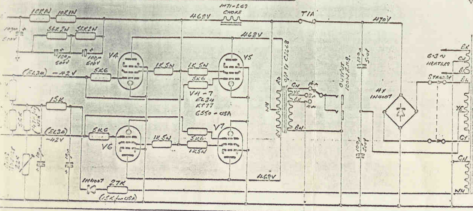
Marshall JCM 810 LEAD SERIES 50W & 100W POWER CIRCUIT DIAGRAM - STANLEY & MASTER VOLUME
