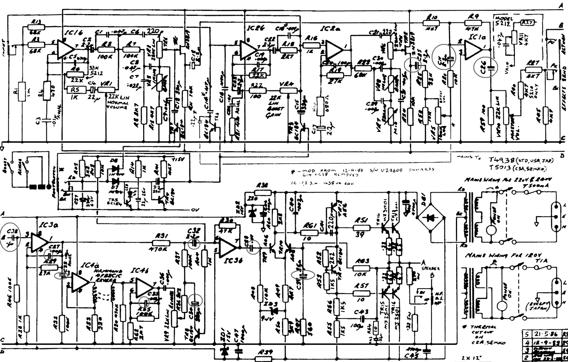
5210 MODEL 5212 50Watt Transistor Reverb Combo - CIRCUIT DIAGRAM
