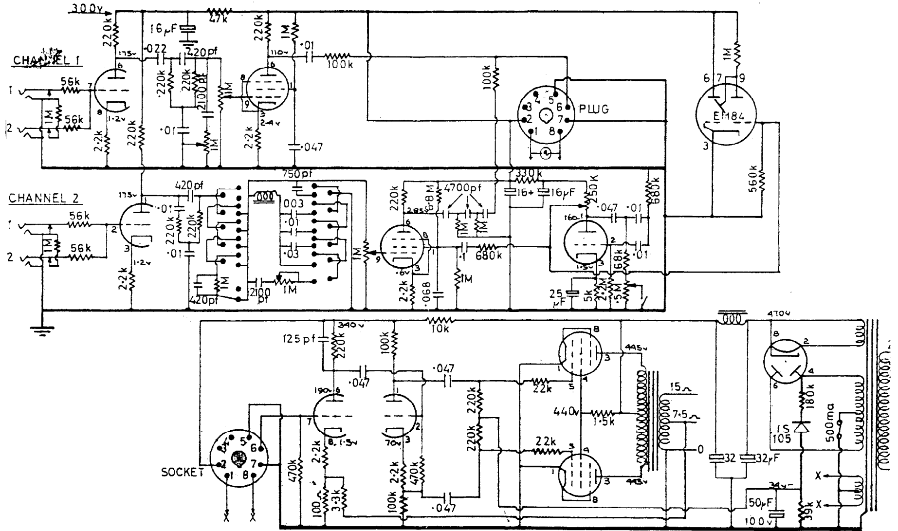
ZODIAC "TWIN 50"
