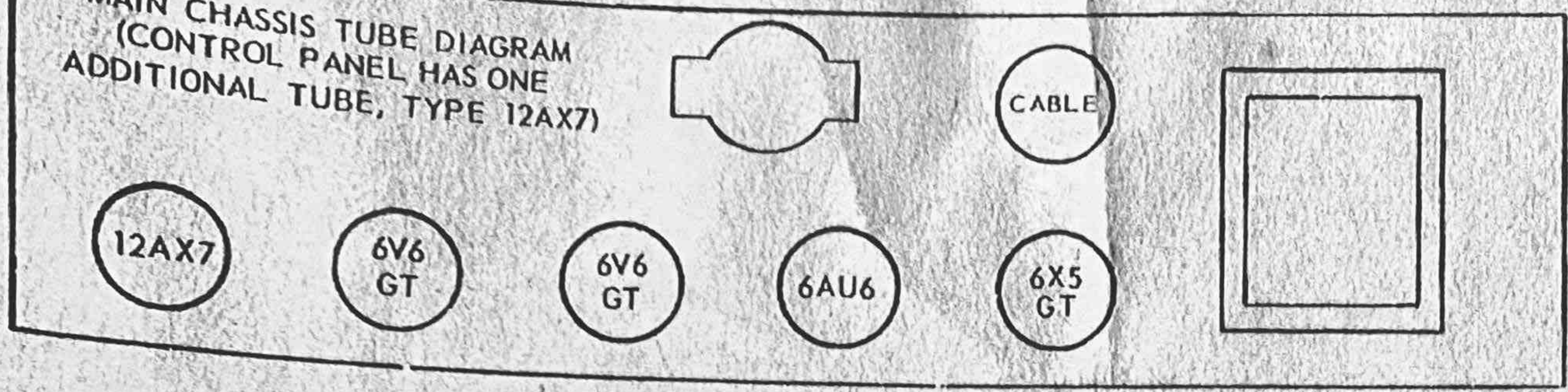
TUBE LAYOUT
