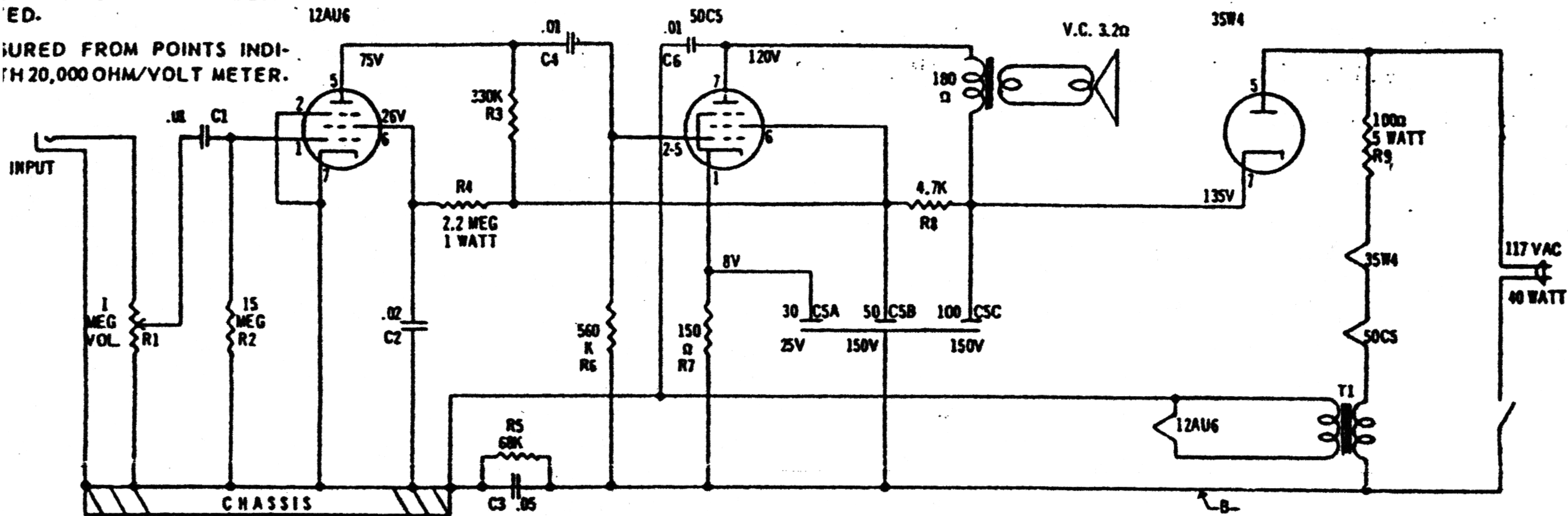
SCHEMATIC DIAGRAM OF SILVERTONE CHASSIS 185.10010
