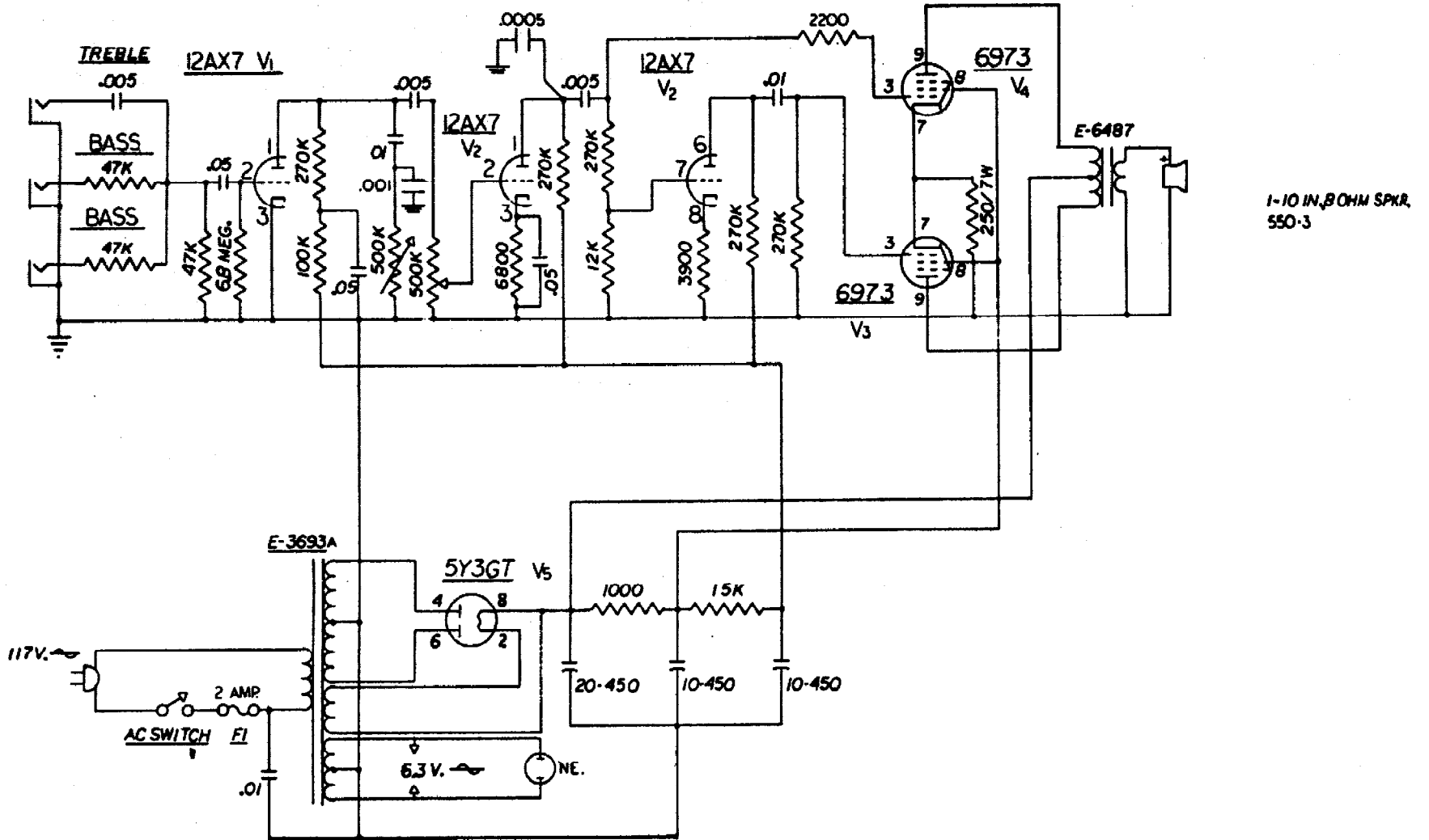
Valco Model 6400
