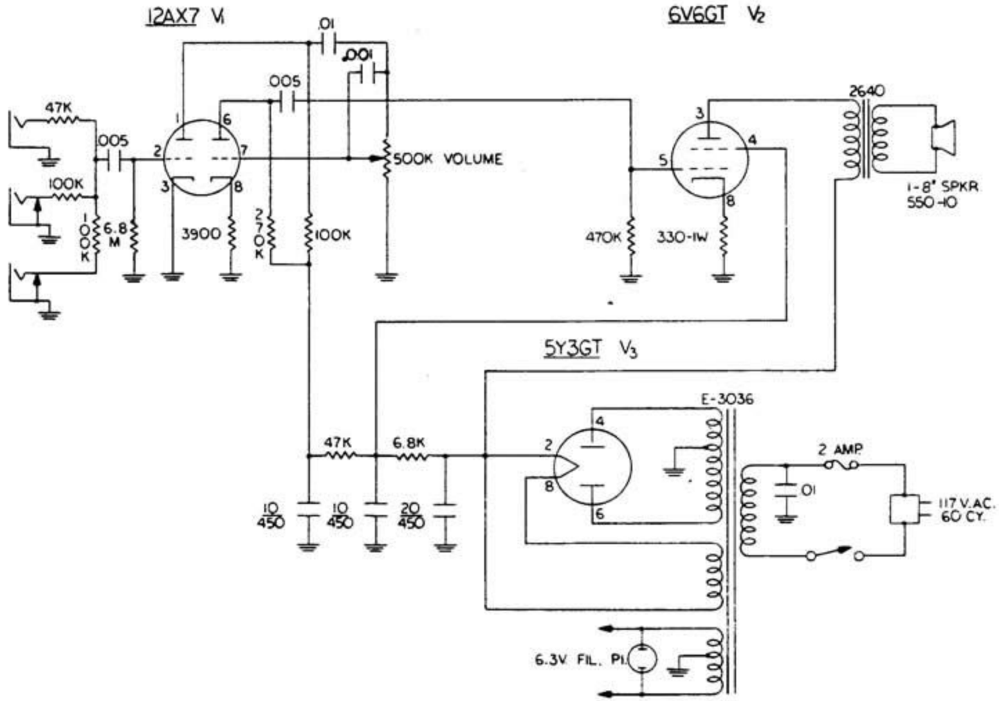
Valco Model 6150
